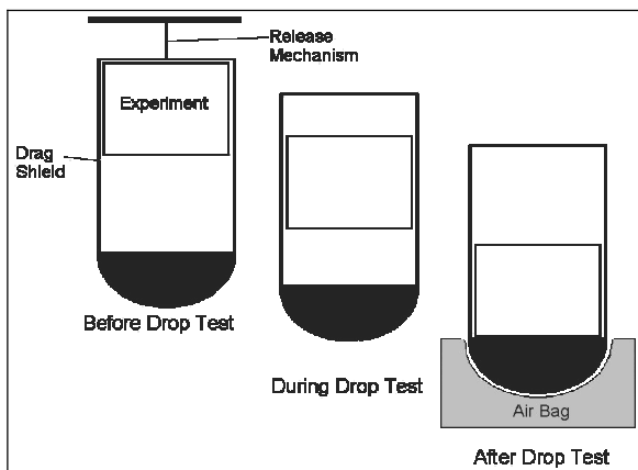
Fig. 2. Drag shield operation
