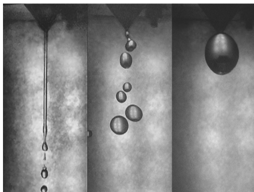
Fig. 6. Different fluid jets and their break-up into drops as observed in reduced gravity: Jetting, chaotic dripping and (attached) quasi-stable growth (left to right, by decreasing velocity)
