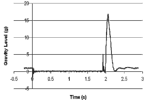
Fig. 3. Gravity level traces for a typical test
