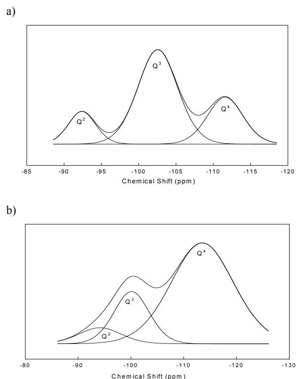
Fig. 7. Deconvoluted NMR spectrum: normal gravity sample (a) and microgravity sample (b)
