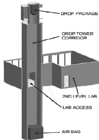
Fig. 1. Schematic of the QUT drop tower
