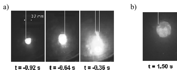
Fig. 4. A metallic rod sample burning in normal gravity (a) and in reduced gravity (b)
