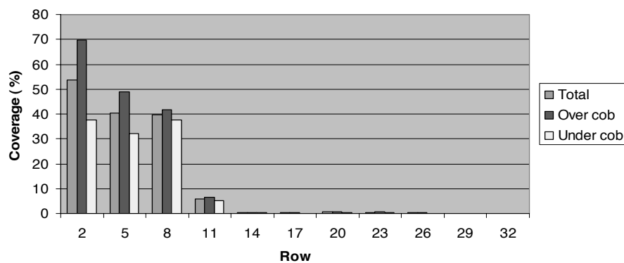
Fig. 9. The total coverage on WSP in experiment with mistblower
