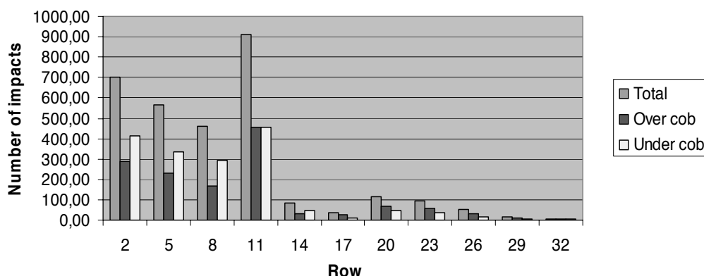
Fig. 13. The number of impacts on WSP in experiment with mistblower
