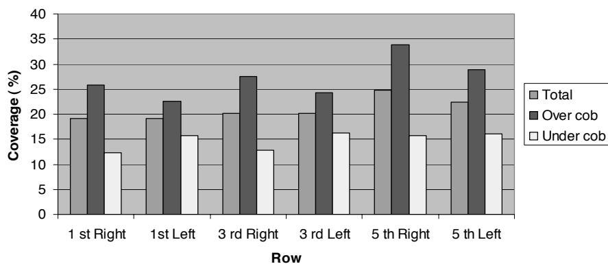
Fig. 8. The total coverage on WSP in experiment with sprayer
