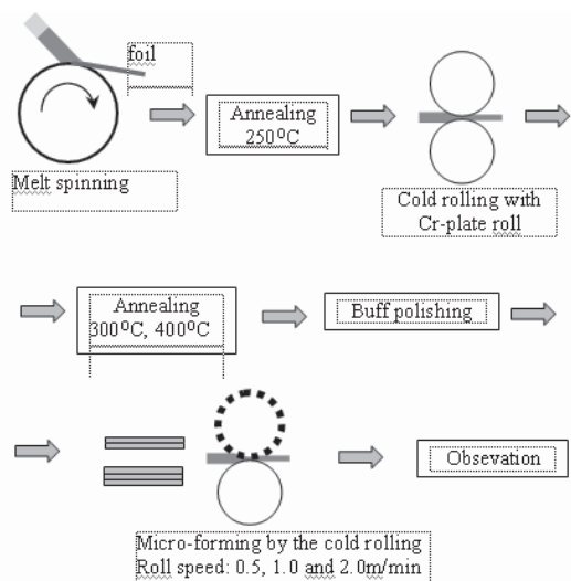
Fig. 4. Schematic illustration showing the process of the foil-casting, the flattening of the foil-surface and micro-forming by the cold rolling
