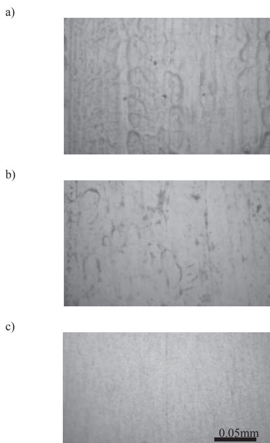
Fig. 5. Surface and roughness of the foil at as-cast, after cold rolling and after buff polishing: a) as-cast condition, roughness Ra: 0.8 \mu m, b) after cold rolling by Cr-plated roll, roughness Ra: 0.5 \mu m, c) after buffing, roughness Ra: 0.3 \mu m
