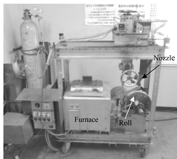
Fig. 1. Nozzle pressing melt spinning method: a) Schematic illustration of the nozzle pressing melt spinning, b) Schematic illustration of enlarged view around the nozzle tip, c) Photograph of the nozzle pressing melt spinning apparatus
