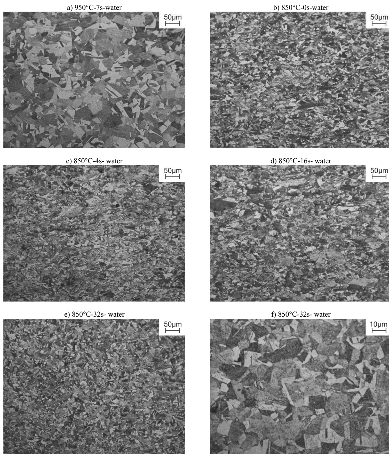
Fig. 16. Austenitic structures obtained after solutioning the steel 27Mn-4Si-2Al-Nb-Ti in successive stages of the hot-working for the specimens compressed to a true strain 4 \times 0.29 and isothermally held for the time from 0 to 64s: a) metadynamically recrystallized grains during the interval between third and fourth deformation, b) initiation of dynamic recrystallization, c) grain refinement due to metadynamic recrystallization, d) grain refinement due to metadynamic and static recrystallization, e, f) fine statically recrystallized austenite grains
