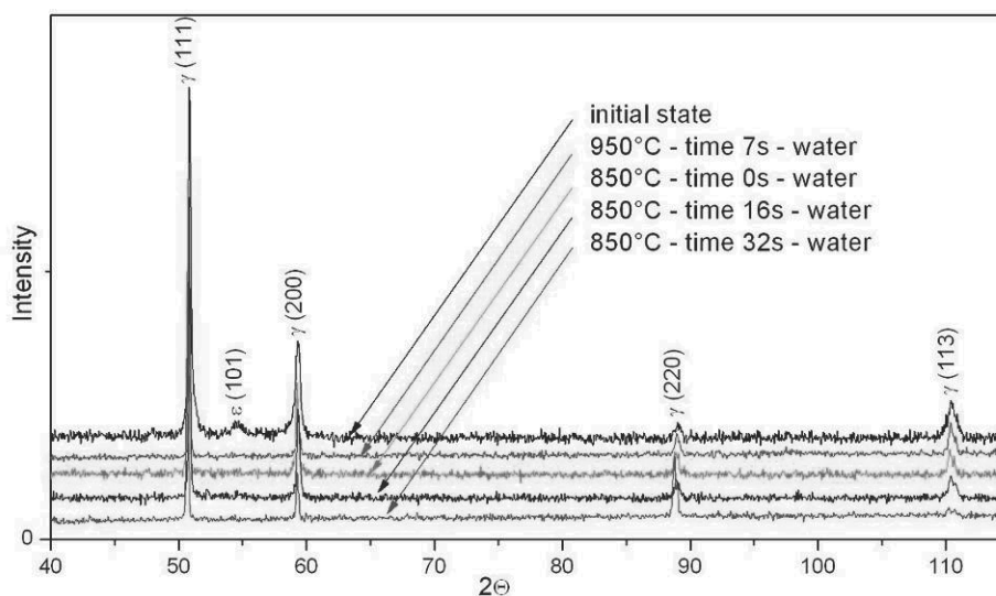
Fig. 18. X-ray diffraction patterns of the steel 27Mn-4Si-2Al-Nb-Ti in the initial state and after different stages of thermo-mechanical treatment
