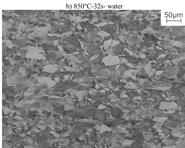
Fig. 24. Fine, statically recrystallized austenite grains and large statically recovered grains of the 26Mn-3Si-3Al-Nb-Ti steel solution heat-treated from a temperature of 850°C after isothermal holding for 32 s of the specimen compressed with the true strain of 4x0.23 (a, b)
