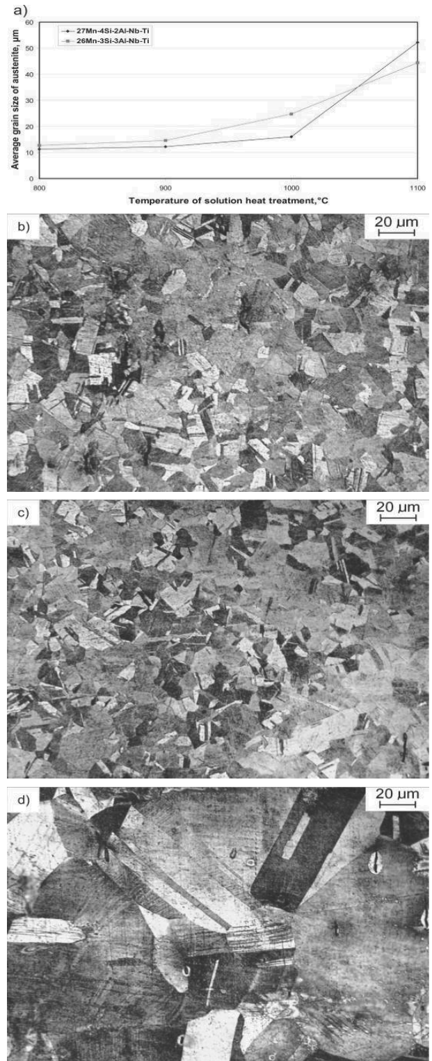
Fig. 4. Changes of austenite grain size in dependence on temperature (a) and structures obtained after solution heat treatment from a temperature: b) 900°C, c) 1000°C, d) 1100°C; 27Mn-4Si-2Al-Nb-Ti steel
