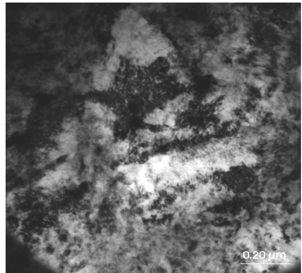
Fig. 17. Regions of dynamically recovered austenite with a various dislocation density of the steel 27Mn-4Si-2Al-Nb-Ti solution heat-treated from a temperature of 850°C directly after the true strain of 4x0.29
