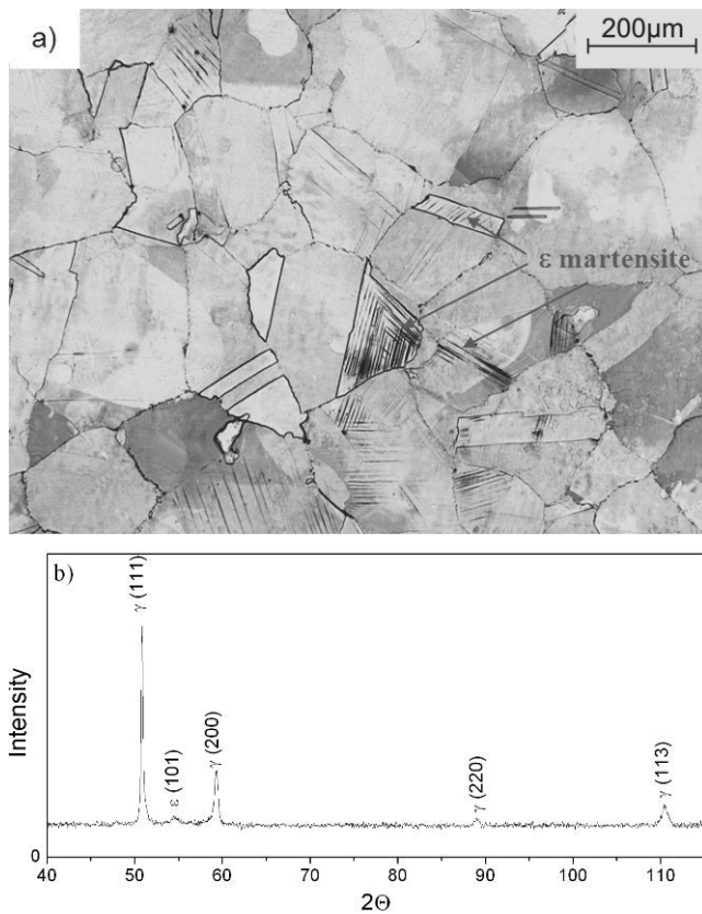
Fig. 3. X-ray diffraction pattern (b) and the austenite structure with many annealing twins and parallel \varepsilon martensite plates of the investigated steel 27Mn-4Si-2Al-Nb-Ti in the initial state (a)
