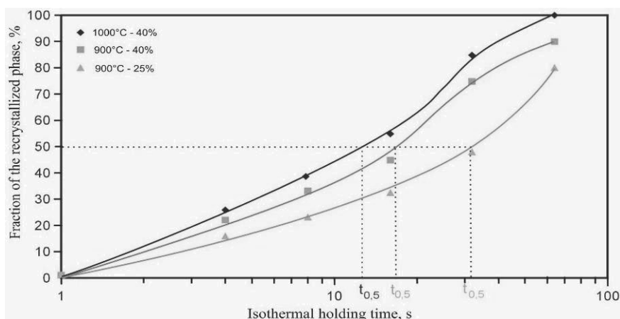
Fig. 11. Progress of recrystallization of the 27Mn-4Si-2Al-Nb-Ti steel isothermally held after plastic deformation in various conditions
