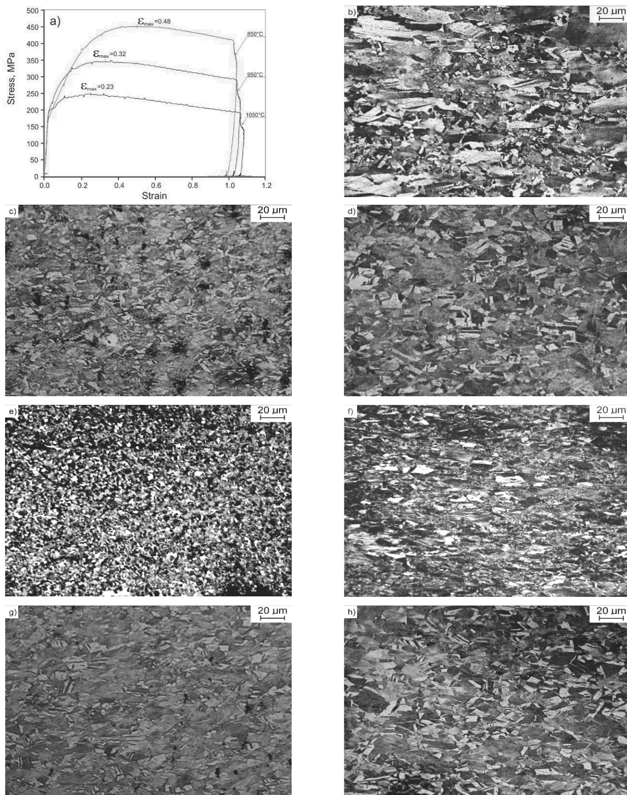
Fig. 6. Evolution of the microstructure of 27Mn-4Si-2Al-Nb-Ti steel compressed to a various strain: a) \sigma - \epsilon curve; b) T = 950^{\circ}\text{C} , \epsilon = 0.5 ; c) T = 950^{\circ}\text{C} , \epsilon = 0.29 ; d) T = 950^{\circ}\text{C} , \epsilon = 0.23 ; e) T = 950^{\circ}\text{C} , \epsilon = 0.91 ; f) T = 850^{\circ}\text{C} , \epsilon = 0.5 ; g) T = 850^{\circ}\text{C} , \epsilon = 0.29 ; h) T = 850^{\circ}\text{C} , \epsilon = 0.23
