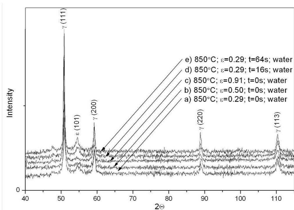
Fig. 10. X-ray diffraction patterns for 27Mn-4Si-2Al-Nb-Ti steel after various variants of the thermo-mechanical treatment; a) 850°C, \varepsilon=0.29 , t=0s , b) 850°C, \varepsilon=0.5 , t=0s , c) 850°C, \varepsilon=0.91 , t=0s , d) 850°C, \varepsilon=0.29 , t=16s , e) 850°C, \varepsilon=0.29 , t=64s
