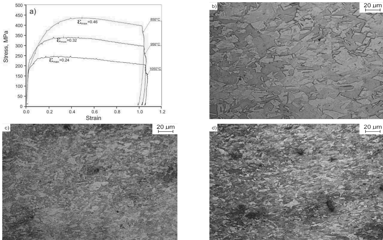
Fig. 7. Evolution of the microstructure of 26Mn-3Si-3Al-Nb-Ti steel compressed to a various strain: a) \sigma - \epsilon curve; b) T = 850^{\circ}\text{C} , \epsilon = 0.23 ; c) T = 850^{\circ}\text{C} , \epsilon = 0.29 ; d) T = 850^{\circ}\text{C} , \epsilon = 0.5
