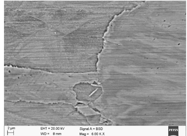
Fig. 22. The fine, statically recrystallized grain on jerky-like boundaries of three large, statically recovered grains of the steel 27Mn-4Si-2Al-Nb-Ti solution heat-treated from the temperature of 850°C after isothermal holding for 32 s of the specimen compressed with the true strain of 4x0.19
