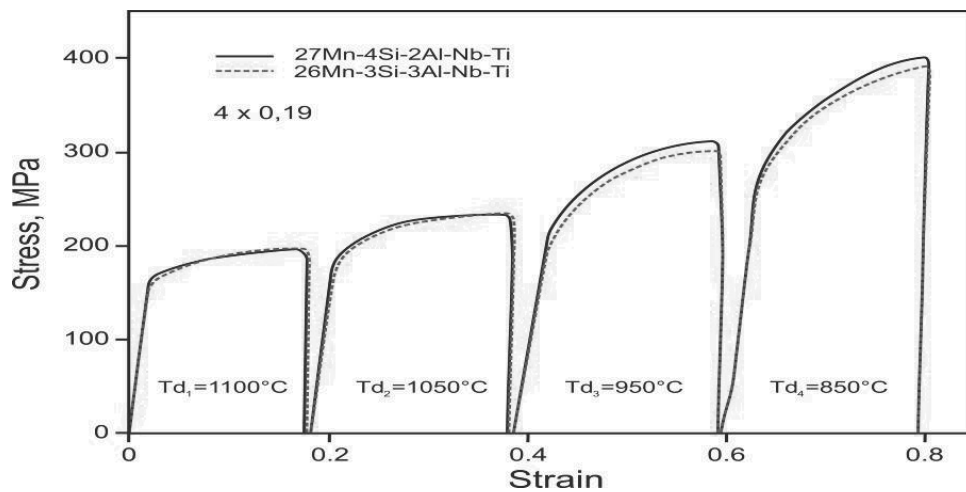
Fig. 15. Stress – strain curves for the specimens plastically deformed 4 \times 0.19
