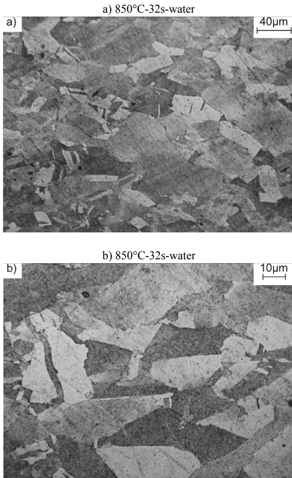
Fig. 21. Fine, statically recrystallized austenite grains and large statically recovered grains of the steel 27Mn-4Si-2Al-Nb-Ti solution heat-treated from the temperature of 850°C after isothermal holding for 32 s of the specimen compressed with the true strain of 4x0.19 (a, b)
