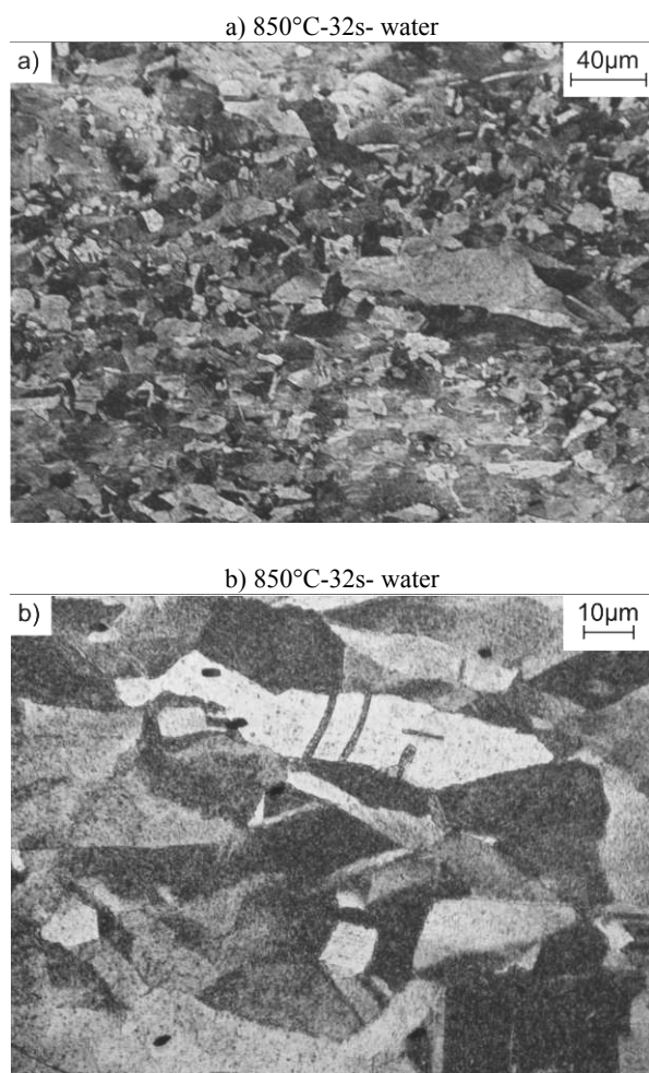
Fig. 19. Fine, statically recrystallized austenite grains and large statically recovered grains of the steel 27Mn-4Si-2Al-Nb-Ti solution heat-treated from a temperature of 850°C after isothermal holding for 32 s of the specimen compressed with the true strain of 4x0.23 (a, b)
