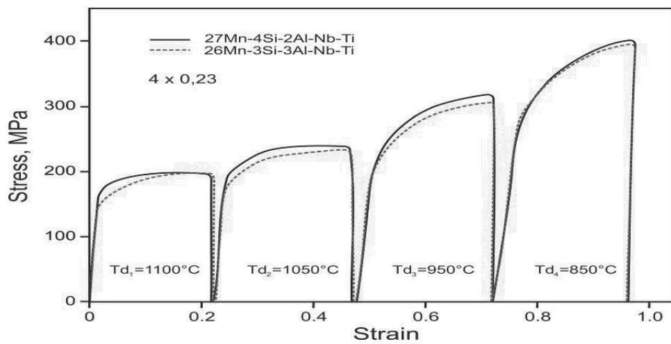
Fig. 14. Stress – strain curves for the specimens plastically deformed 4 \times 0.23
