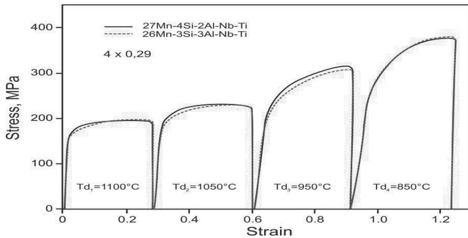
Fig. 13. Stress – strain curves for the specimens plastically deformed 4 \times 0.29
