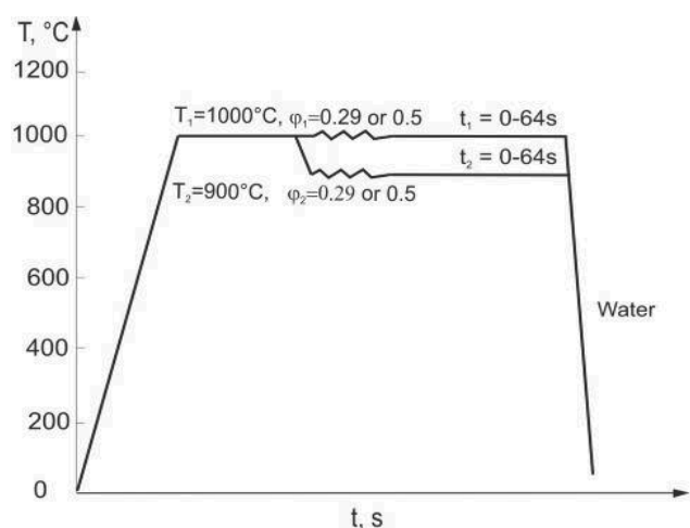
Fig. 1. Parameters of the preliminary hot upsetting tests
