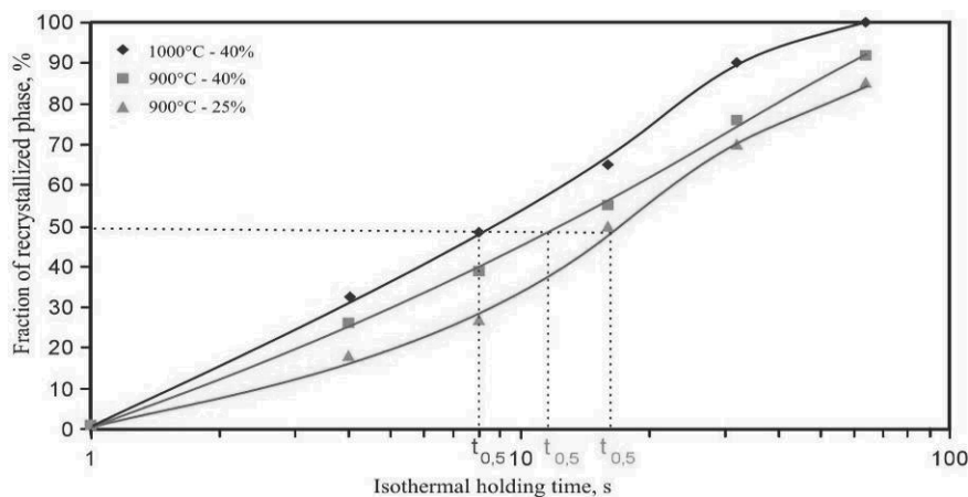
Fig. 12. Progress of recrystallization of the 26Mn-3Si-3Al-Nb-Ti steel isothermally held after plastic deformation in various conditions
