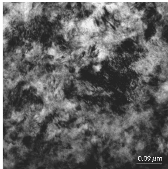
Fig. 20. Regions of statically recovered austenite with a various dislocation density of the steel 27Mn-4Si-2Al-Nb-Ti solution heat-treated from the temperature of 850°C after isothermal holding for 32 s of the specimen compressed with the true strain of 4x0.23
