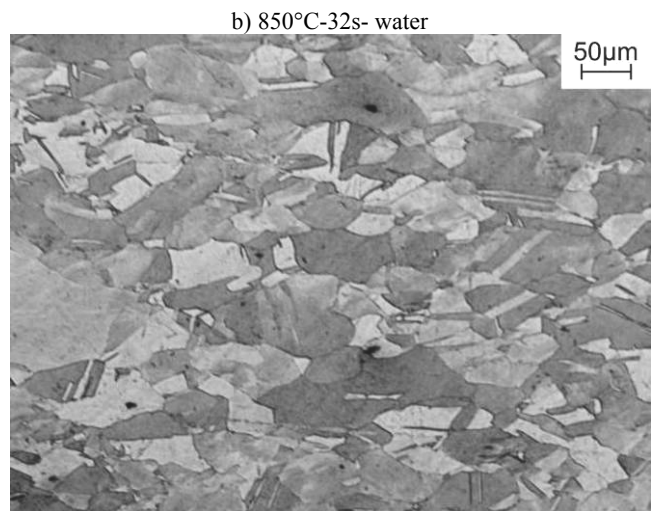
Fig. 25. Fine, statically recrystallized austenite grains and large statically recovered grains of the 26Mn-3Si-3Al-Nb-Ti steel solution heat-treated from the temperature of 850°C after isothermal holding for 32 s of the specimen compressed with the true strain of 4x0.19 (a, b)
