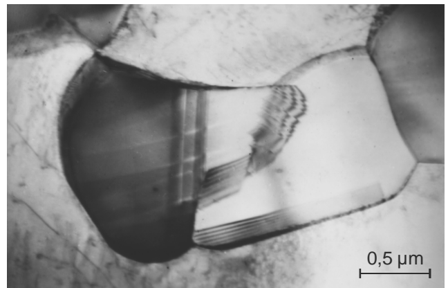
Fig. 34. Microstructure within approx. 0.15 mm from the X40CrMoV5-1 steel surface borided at 1030°C for 4 hrs; thin foil
