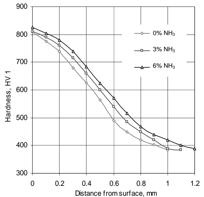
Fig. 27. Hardness distribution in a surface layer of 18CrMnTi4-4 steel after carburising and carbonitriding with addition of 3 and 6% of \text{NH}_3 , at temperature of 880°C for 5 hrs and quenching from 840°C
