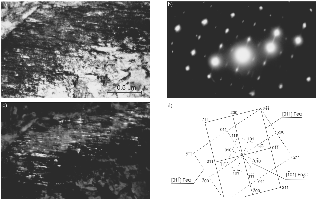
Fig. 28. Surface layer microstructure of 18CrMnTi4-4 steel after carburising at temperature of 880°C, quenching from 840°C and tempering at 300°C, thin foil, a – bright field image, b – diffraction pattern from the area as in Fig. a, c – dark field image from 111 M_3C reflection, d – diffraction pattern solution from Fig. b
