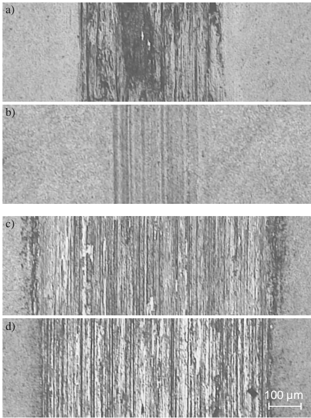
Fig. 20. Wear tracks formed in a pin-on-disc test on X37CrMoV5-1 steel: a) and c) heat treated steel, b) and d) plasma-nitrided steel; a test for 7500 revolutions at a temperature of a) and b) 20°C, and c) and d) 500°C
