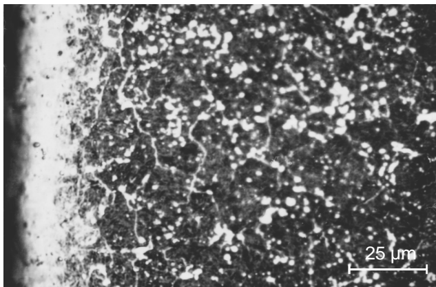
Fig. 9. Surface layer microstructure of HS6-5-2 steel quenched, tempered and gas-nitrided at 570°C for 4 hrs in an ammonia atmosphere
