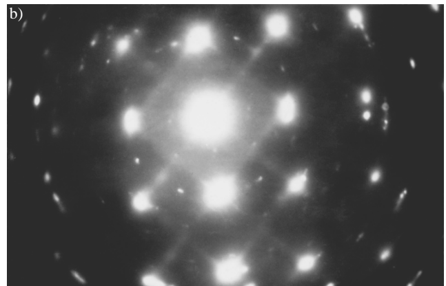
Fig. 8. Surface layer microstructure of 38CrAlMo6-10 steel quenched from 920°C, tempered at 575°C and gas-nitrided at 570°C for 8 hrs in an ammonia atmosphere
