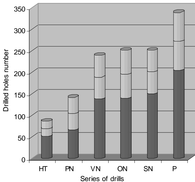
Fig. 29. Cutting ability tests results for drills made of HS6-5-2 steel that was heat treated (HT) and plasma nitrided (PN), sulphonitrided and vacuum nitrided (VN), oxynitrided in fluidised bed (ON), nitrided selectively (SN) and passivated in water vapour (P)
