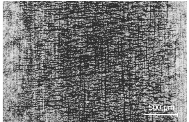
Fig. 22. Cracks at the surface of the X40CrMoV5-1(vac) steel specimen quenched from 1030°C and tempered at 600°C, formed during 5000 thermal cycles within 600-100°C with induction heating
