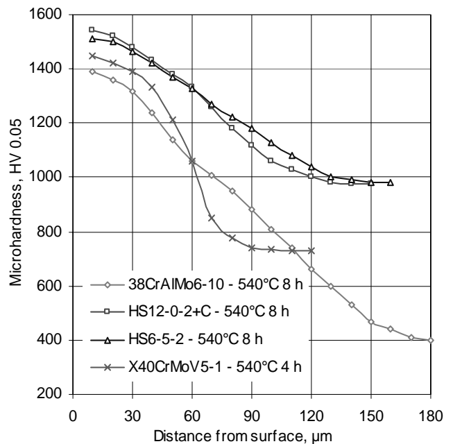
Fig. 7. Microhardness distribution in the surface layer of the selected steels subject to quenching and tempering gas nitriding at 540°C
