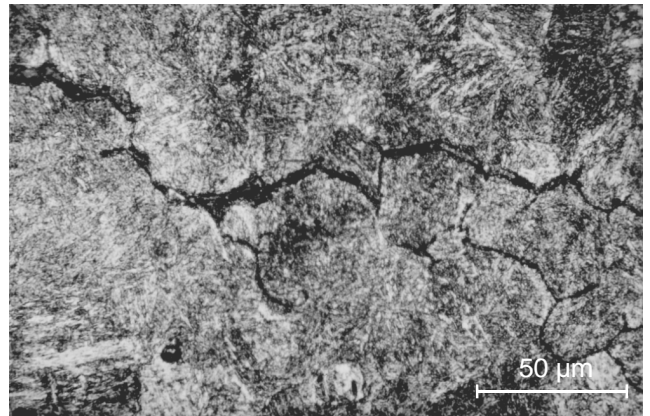
Fig. 23. Microstructure within approx. 0.5 mm from the 38CrMoVB10-4 steel specimen quenched from 890°C and tempered at 500°C, after 3000 thermal cycles within 600-100°C
