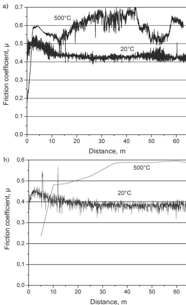
Fig. 19. Variation curve of the friction coefficient according to the friction path length for a) thermal treated and b) plasma-nitrided X37CrMoV5-1 steel tested at a temperature 20^\circ\text{C} and 500^\circ\text{C} for 1000 revolutions
