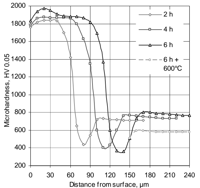
Fig. 32. Microhardness distribution in the surface layer of X40CrMoV5-1 steel borided at temperature of 1030°C for 2 to 6 hrs and directly quenched and tempered twice at 600°C
