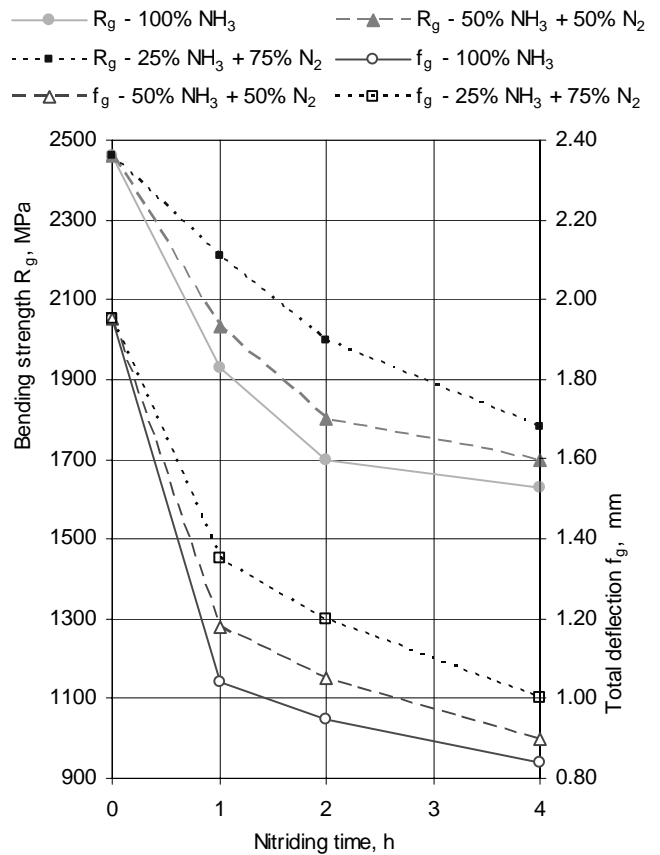
Fig. 13. Influence of nitriding conditions on the properties identified in the static bending test of the specimens made of HS6-5-2 steel quenched, tempered and gas-nitrided at 540°C
