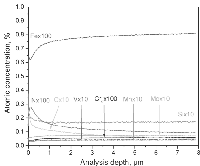
Fig. 18. Variations in the concentration of elements in plasma-nitrided X37CrMoV5-1 steel analysed with a GDOES spectrometer
