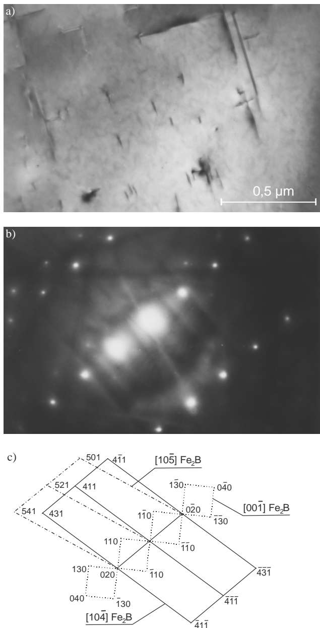
Fig. 33. Dislocation in a \text{Fe}_2\text{B} boride grain within approx. 0.08 mm from the surface of X40CrMoV5-1 steel borided at 1030°C for 6 hrs; thin foil, a – bright field image, b – diffraction pattern from the area as in Fig. a, c – diffraction pattern solution from Fig. b
