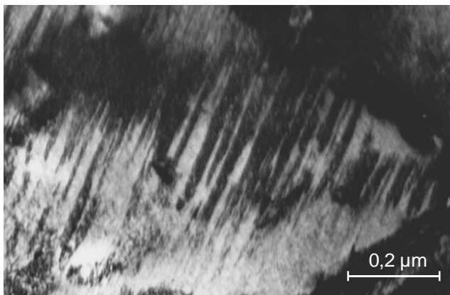
Fig. 26. Microstructure of the surface layer of 18CrMnTi4-4 steel after carbonitriding with addition of 6% of \text{NH}_3 at a temperature of 880°C and quenching from 840°C, thin foil
