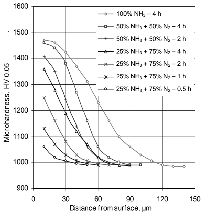
Fig. 11. Microhardness distribution in the surface layer of HS6-5-2 steel quenched from 1230°C, tempered at 550°C and gas-nitrided at 540°C in an atmosphere of ammonia with addition of nitrogen
