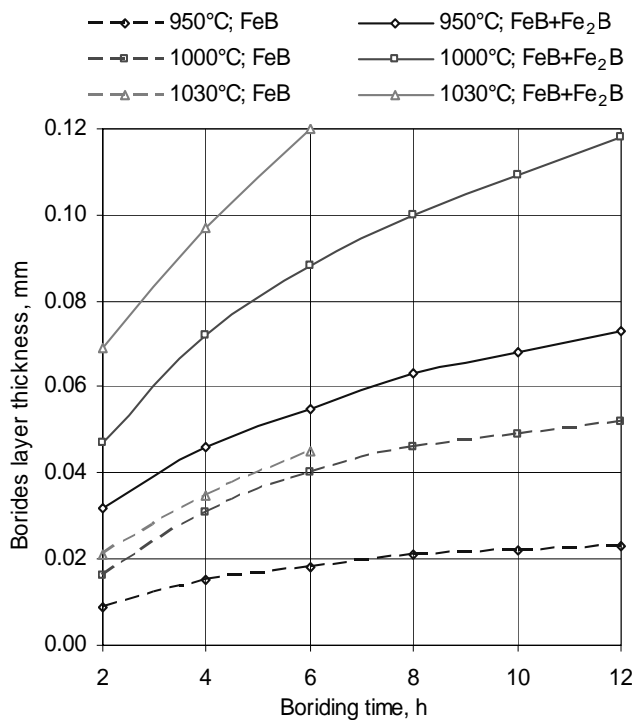
Fig. 31. Effect of boriding temperature and duration on borides layer thickness on X40CrMoV5-1 steel
