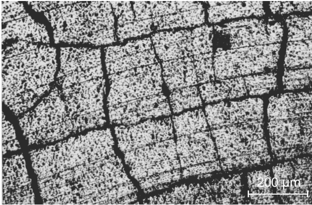
Fig. 35. Cracks lattice at the surface of the X40CrMoV5-1 steel specimen borided at a temperature of 950°C for 8 hrs, quenched from 1030°C and tempered twice at 600°C, formed during 25000 thermal cycles within 600-20°C
