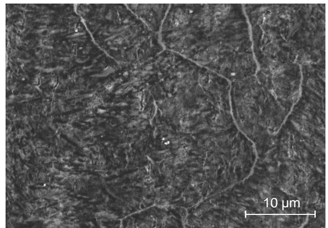
Fig. 16. Microstructure of the plasma-nitrided surface layer of X37CrMoV5-1 steel, SE image
