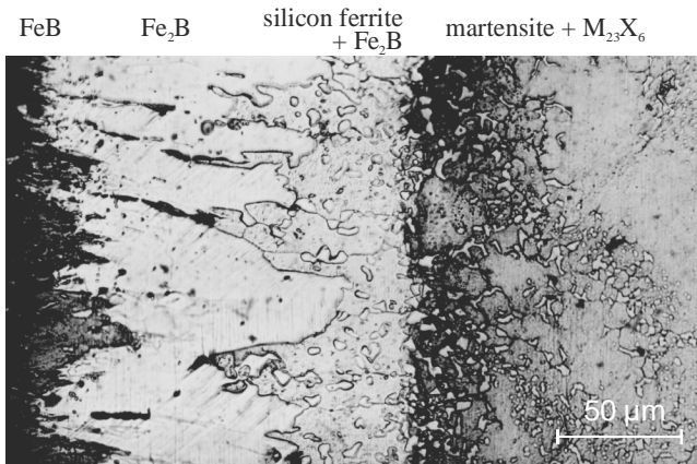
Fig. 30. Elongation of FeB and Fe 2 B boride grains in the surface layer of X40CrMoV5-1 steel borided at 1030°C for 6 hrs
