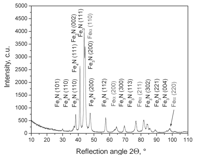
Fig. 17. X-ray diffraction pattern of the plasma-nitrided surface layer of X37CrMoV5-1 steel
