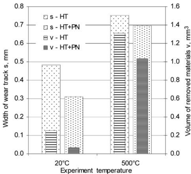
Fig. 21. Width of wear tracks and the volume of the removed material for heat treated (HT) and plasma-nitrided X37CrMoV5-1 steel (PN), subject to a pin-on-disc test (after 7500 revolutions)
