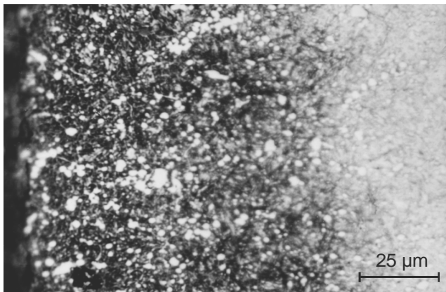
Fig. 12. Surface layer microstructure of HS6-5-2 steel gas-nitrided at 540°C for 4 hrs in an atmosphere containing 25% NH 3 and 75% N 2
