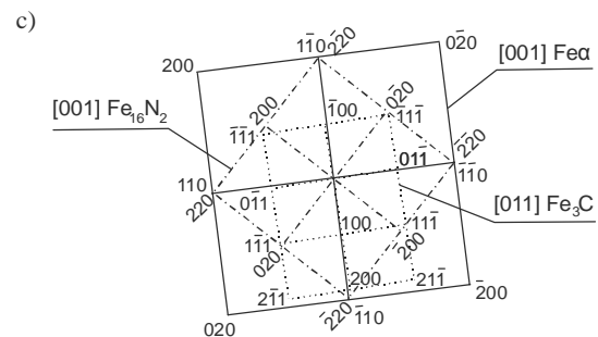
Fig. 10. Surface layer microstructure of HS6-5-2 steel quenched, tempered and gas-nitrided at 540°C for 3 hrs; thin foil, a – bright field image, b – diffraction pattern from the area as in Fig. a, c – diffraction pattern solution from Fig. b
