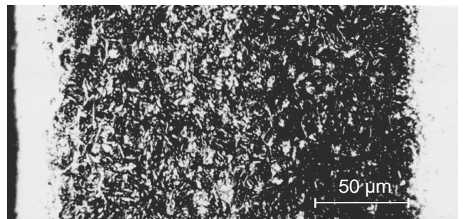
Fig. 14. Microstructure of the X40CrMoV5-1 steel surface layer gas-nitrided at 570°C for 6 hrs
