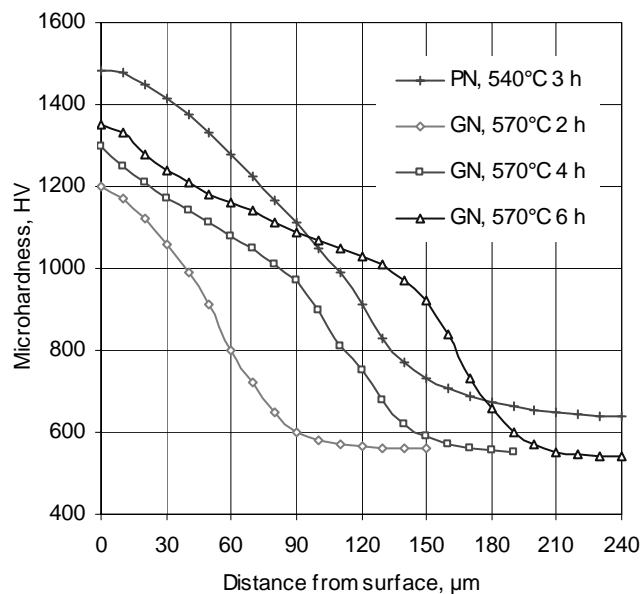
Fig. 15. Microhardness distribution in the surface layer of gas-nitrided X40CrMoV5-1 steel (GN) and plasma-nitrided X37CrMoV5-1 steel (PN)
