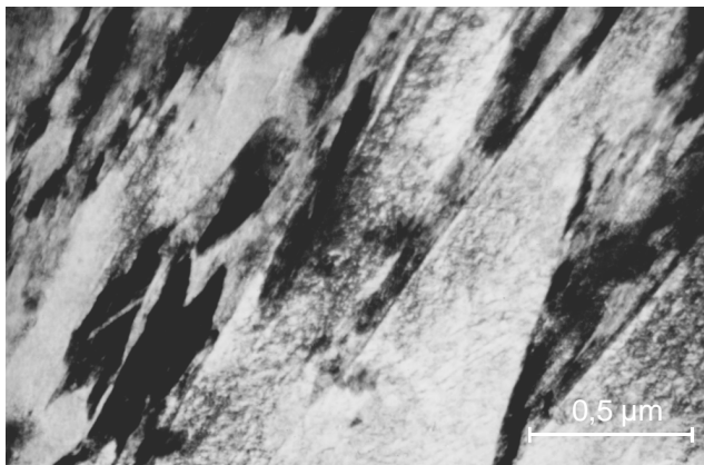
Fig. 25. Microstructure of the surface layer of 18CrMnTi4-4 steel after carburising at a temperature of 880°C and quenching from 840°C, thin foil
