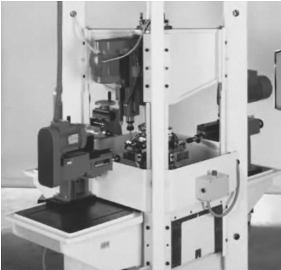
Fig. 1. A typical SPM for performing drilling and tapping operations [11]
