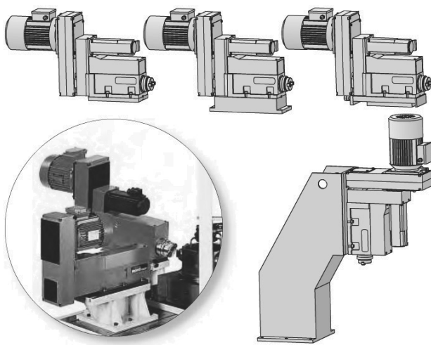
Fig. 5. Assembly equipment for positioning machining units [11]
