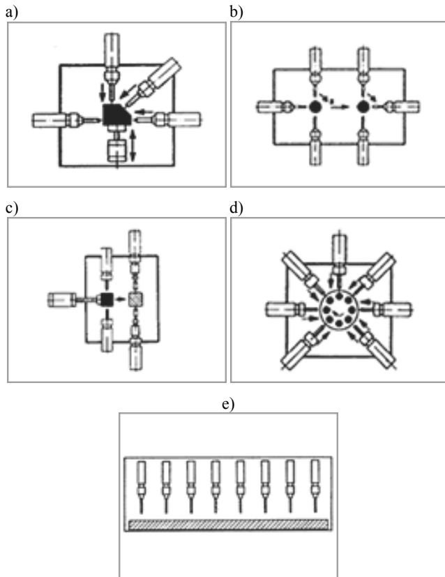
Fig. 7. SPM layouts for a) single-station, b) special application, c) transfer machine, d) rotary machine, e) in-line drilling [11]
