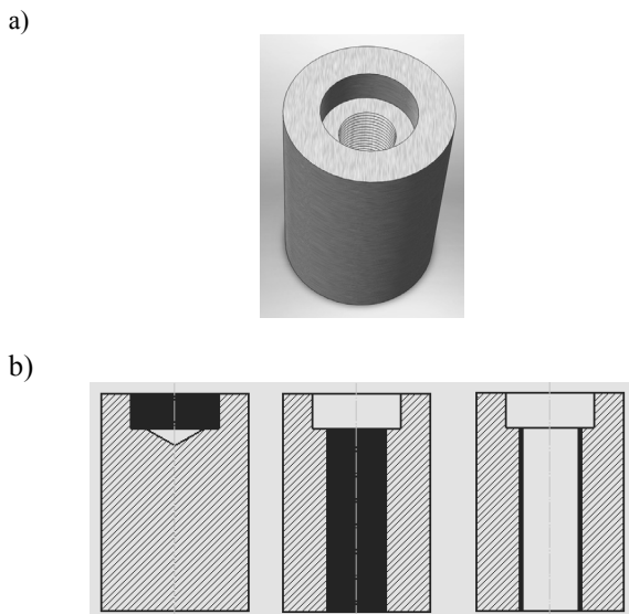
Fig. 10. a) Part with three machining features, b) operations from left to right: counterboring, drilling, and tapping
